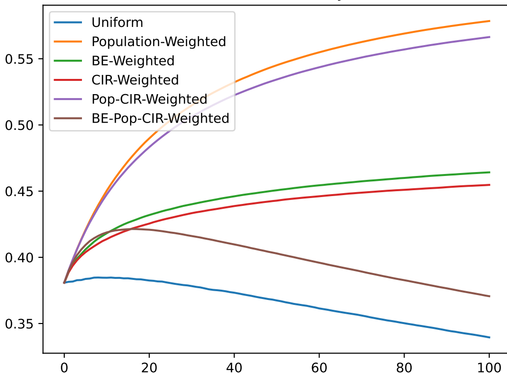
SD, 2000: Blue Player
